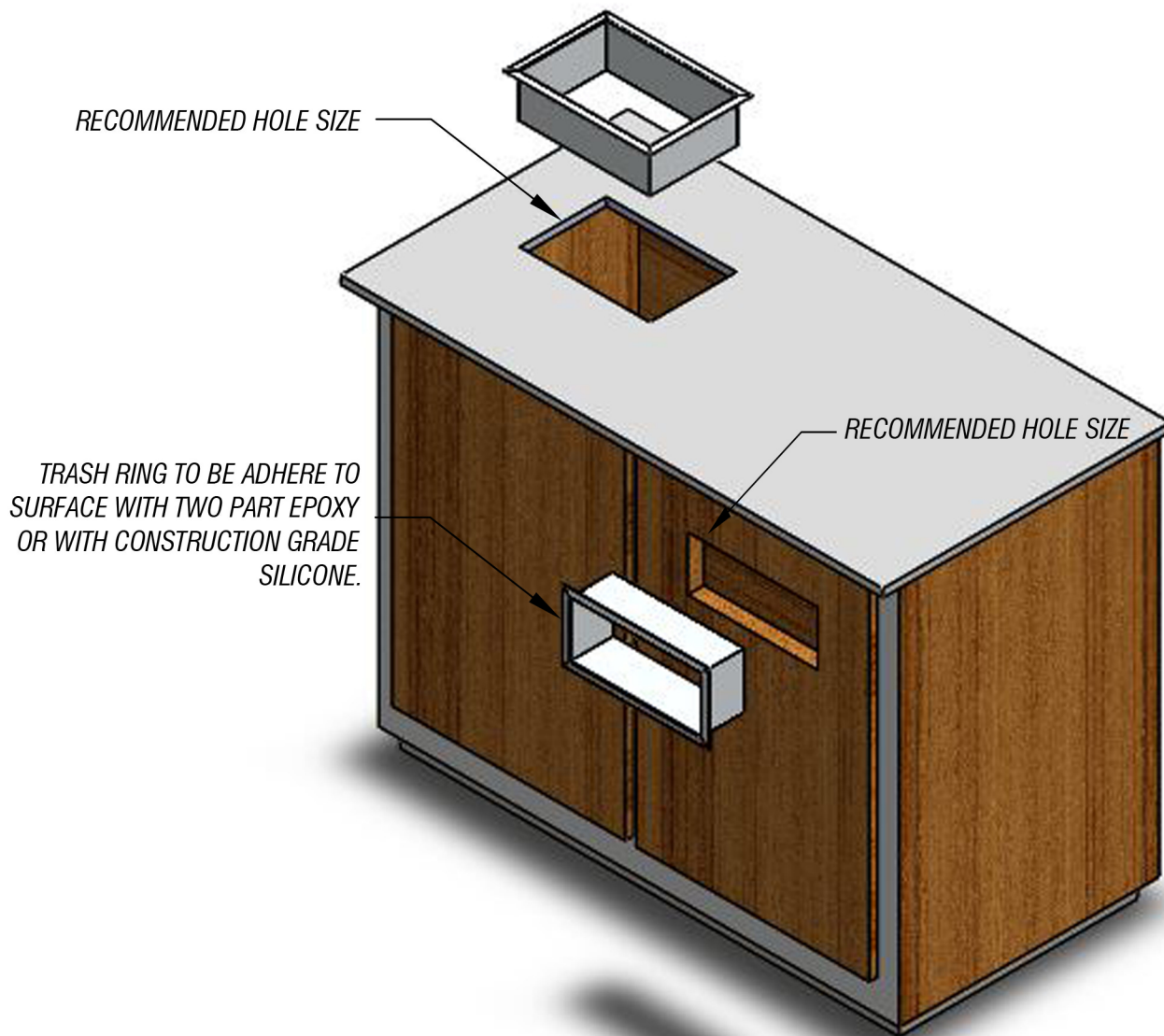
ISOMETRIC VIEW
