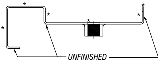
FINISH DETAIL
