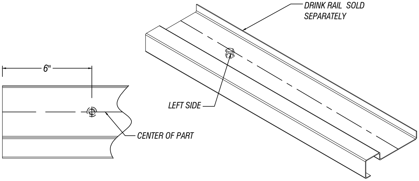
TOP VIEW
