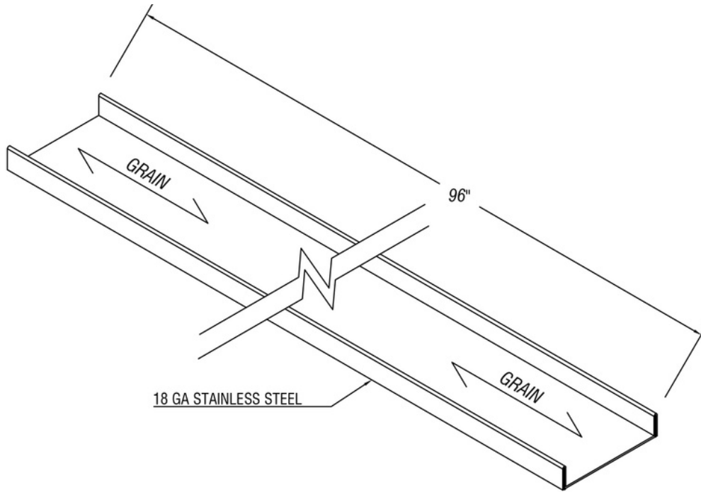
ISOMETRIC VIEW
