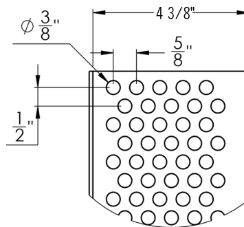
DETAIL-1
