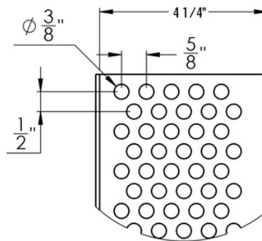
DETAIL-1
