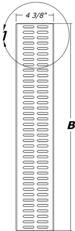
TOP VIEW
