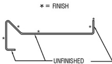
FINISH DETAIL
