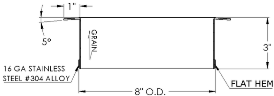
SECTION VIEW
