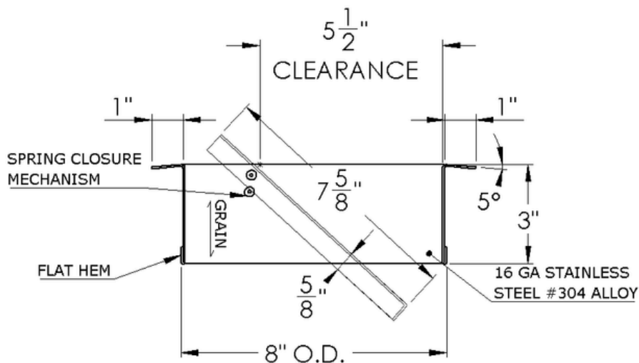
SECTION VIEW
