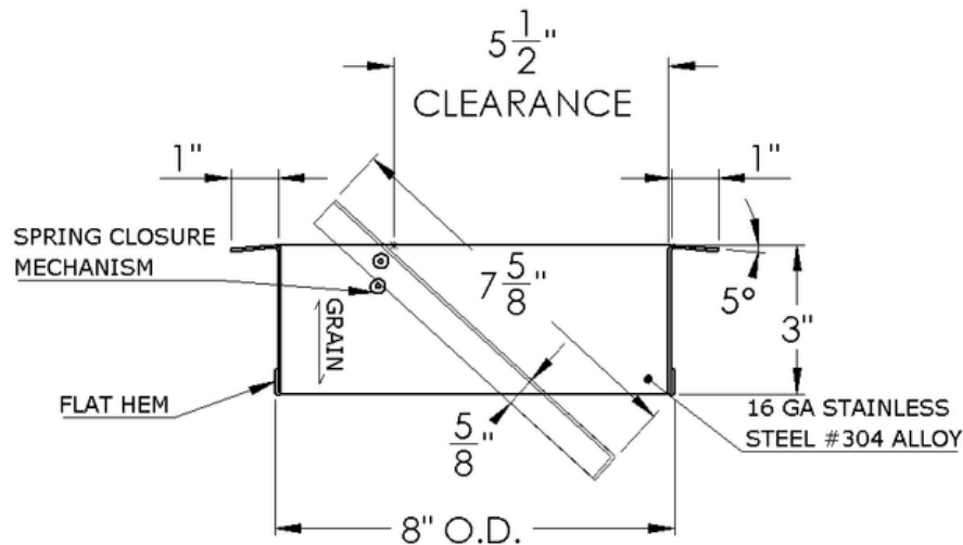
SECTION VIEW
