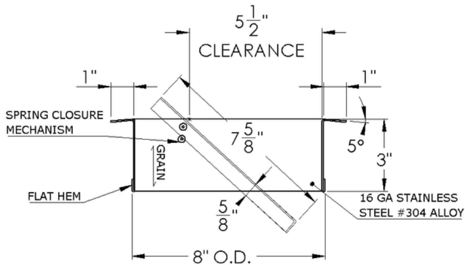
SECTION VIEW
