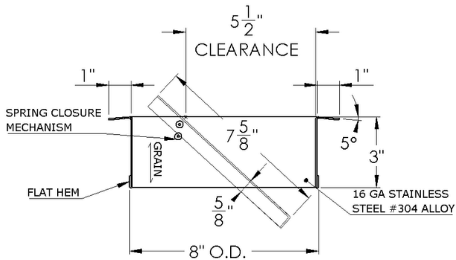
SECTION VIEW
