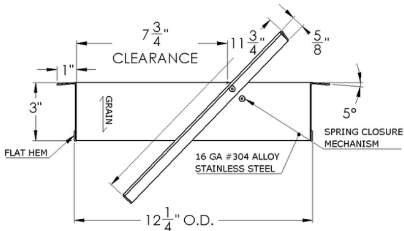
SECTION VIEW
