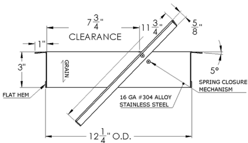
SECTION VIEW
