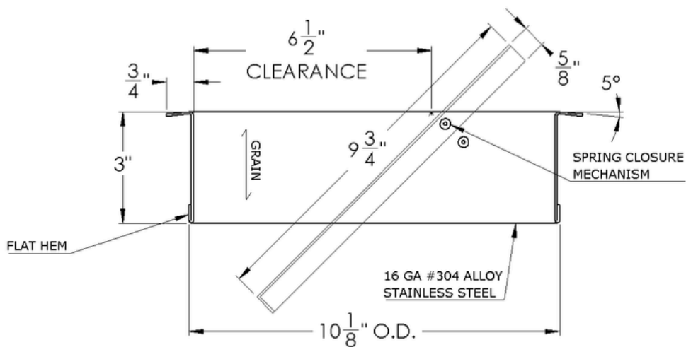
SECTION VIEW
