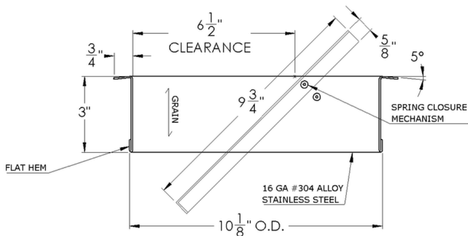
SECTION VIEW
