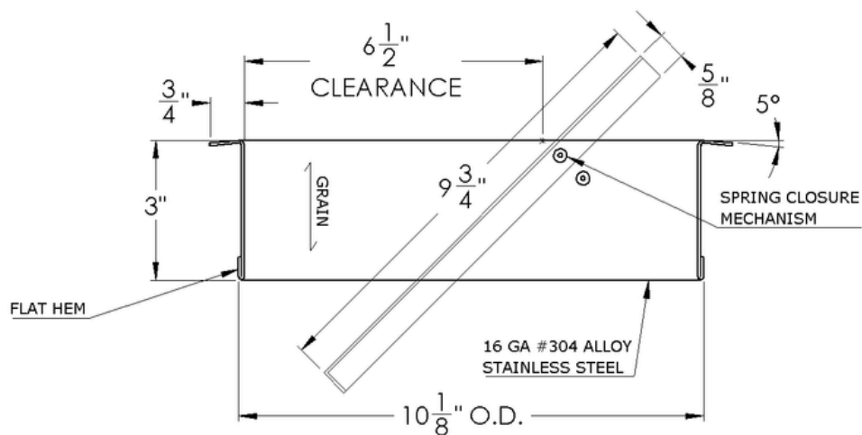
SECTION VIEW
